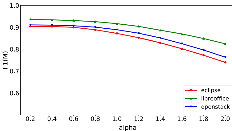
Fig. 11 Sensitivity of F1-score for merged code changes, i.e., F1(M), of our approach to the choice of \alpha for Eclipse, LibreOffice and OpenStack datasets
